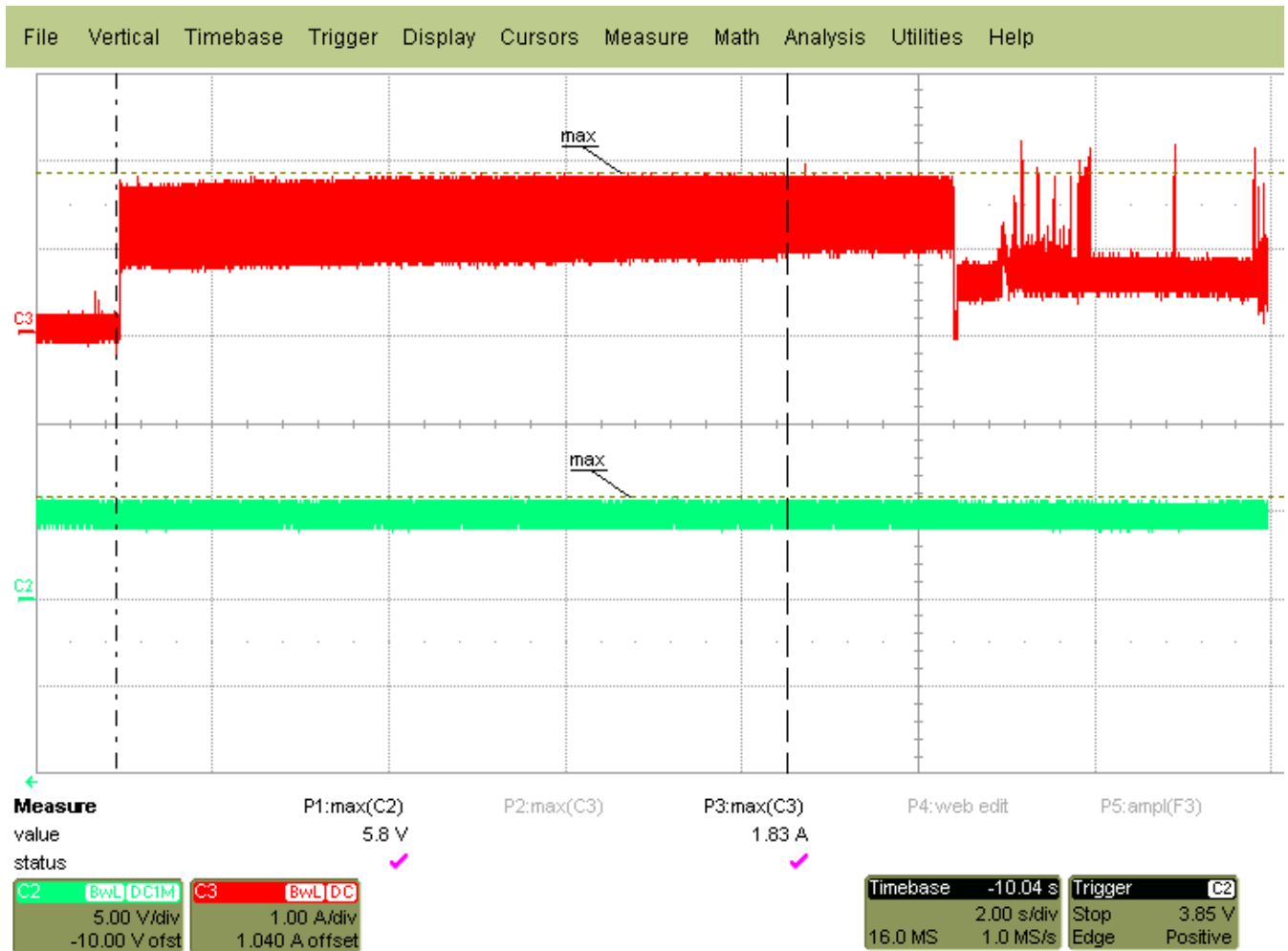
Figure 1 8TB Typical 5V and 12V startup and operation current profiles
