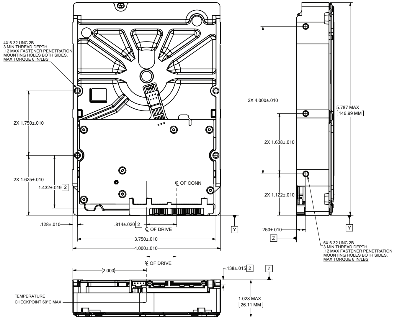
Figure 3 Mounting dimensions (6TB model)
