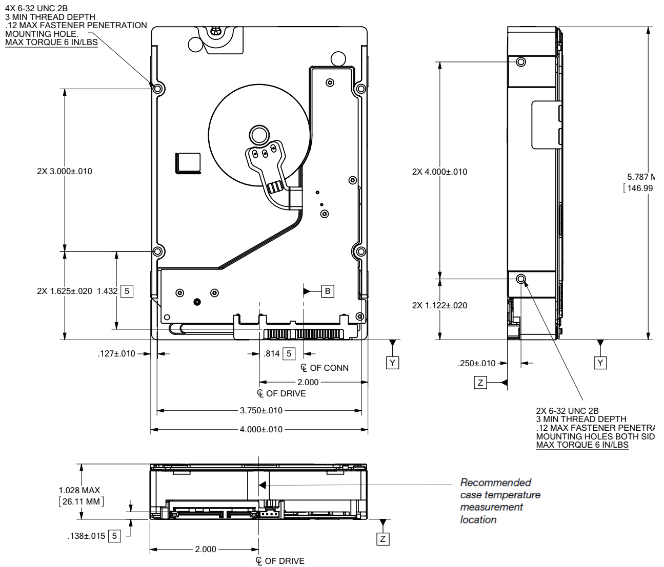
Figure 4 Mounting dimensions (8TB model).
